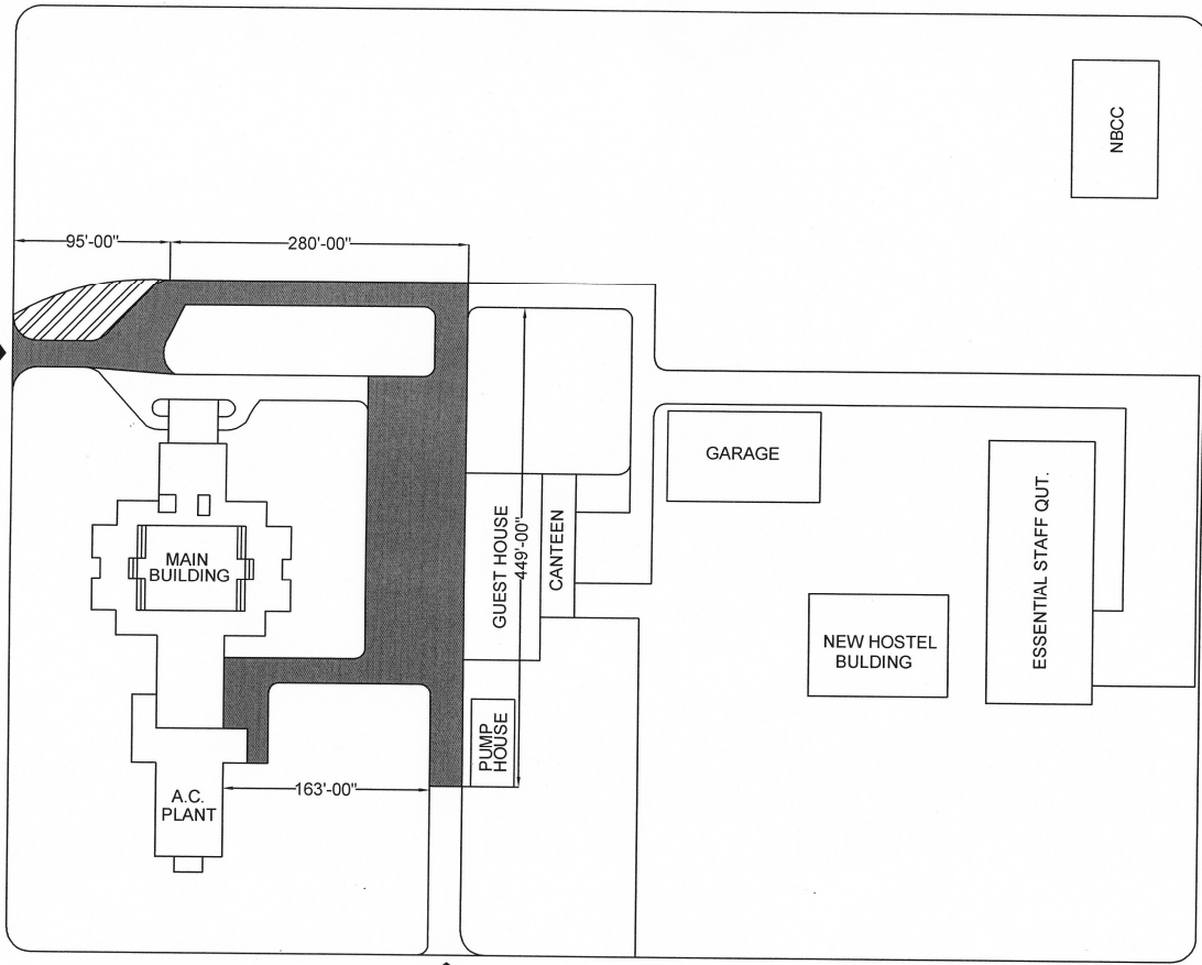
LAYOUT PLAN OF INSIDE CAMPUS ROAD
