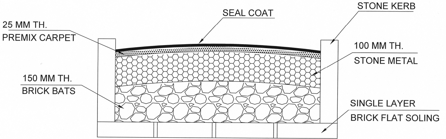
TYPICAL SECTION OF ROAD
